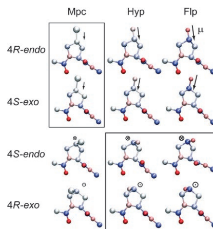
Figure 2. Optimized geometries of the L-proline derivatives as trans amide conformers: The strength and direction of the X–C γ bond dipoles \mu are indicated by arrows. The atomic partial charges are indicated by a color code ranging from red (negative) through white (neutral) to blue (positive); adjacent red and blue atoms represent dipoles. The spheres represent “compound atoms”; the charges of hydrogen atoms are added to those of the neighboring heavy atoms. The experimentally observed conformers are marked by boxes.
