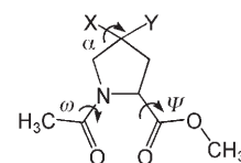
Figure 1. Chemical structure of N -acetylproline methyl ester ( 4 , X = Y = H) and various derivatives, in which either X or Y is replaced by SH ( 1 ), SMe ( 2 ), SSMe ( 3 ), OH ( 5 ), or F ( 6 ).
